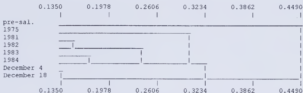
Figure 3. Classification of 8 waterbird surveys at Toolibin Lake, based on species composition. The pre-salinization survey contains composite data from 1965-74 and the December surveys were conducted in 1996.
